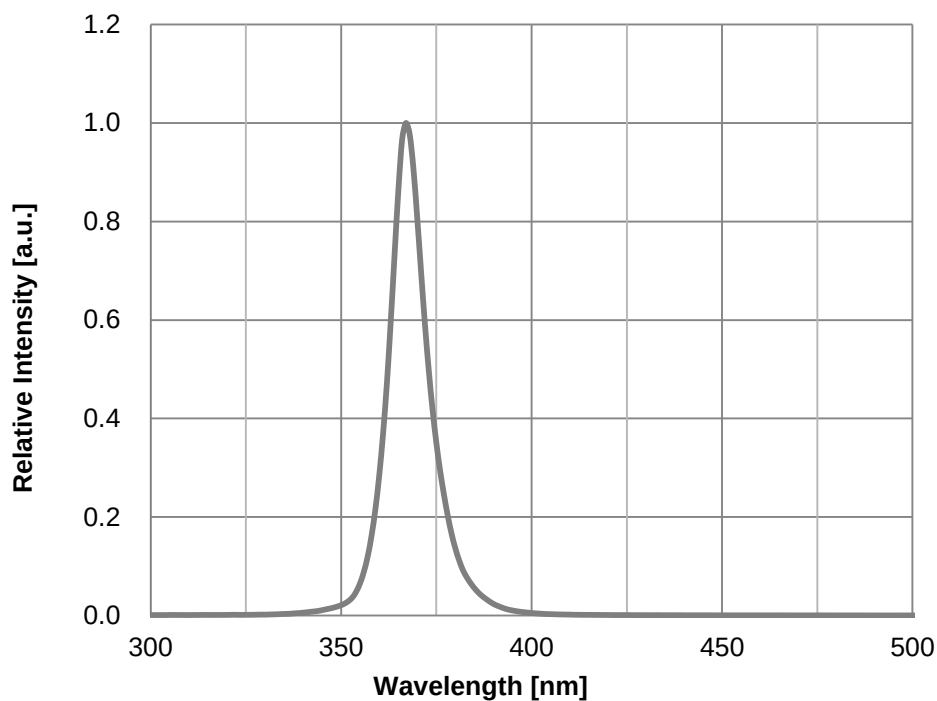
Fig 1. Spectrum, T_s=25^{\circ}\text{C} , I_F=250\text{mA}
