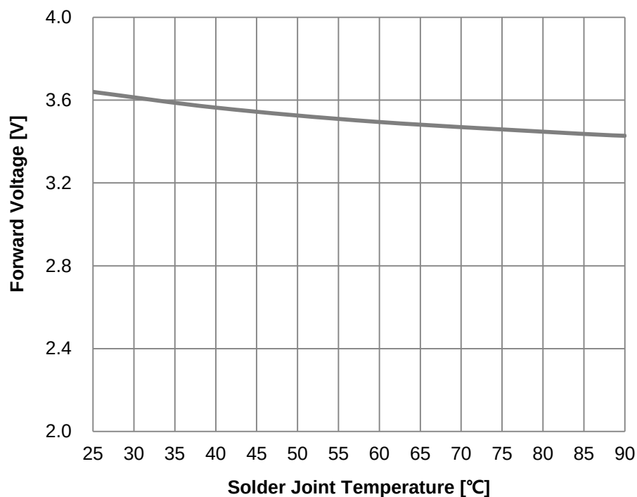
Fig 7. Solder Joint Temperature vs. Forward Voltage, I_F=250\text{mA}
