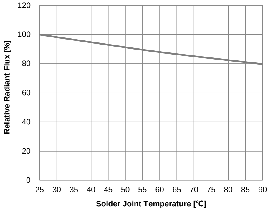
Fig 5. Solder Joint Temperature vs. Relative Radiant Flux, I_F=250\text{mA}
