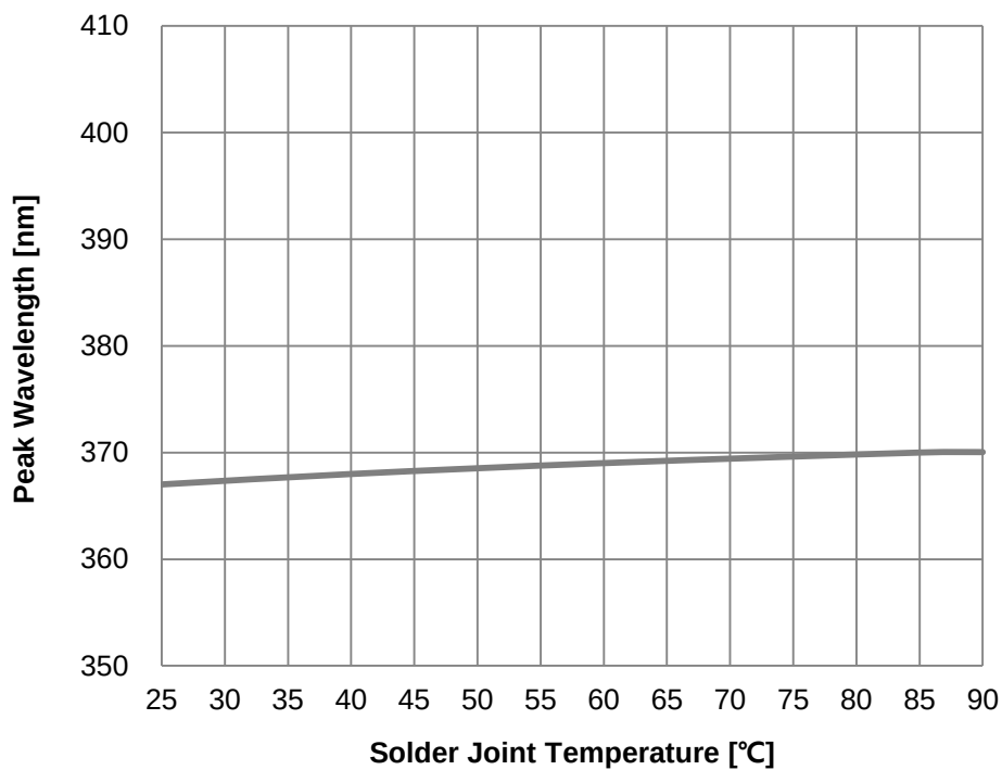
Fig 6. Solder Joint Temperature vs. Peak Wavelength, I_F=250\text{mA}
