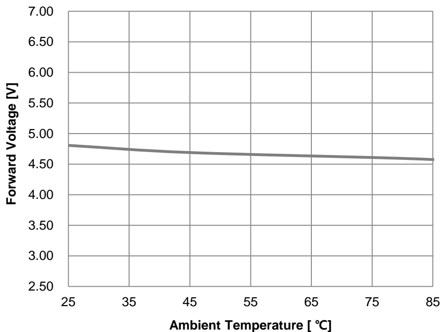
Fig 7. Ambient Temperature vs. Forward Voltage, I_F=150\text{mA}
