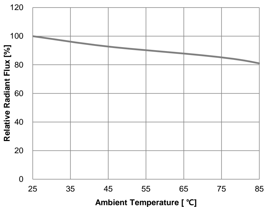
Fig 5. Ambient Temperature vs. Relative Radiant Flux, I_F=150\text{mA}
