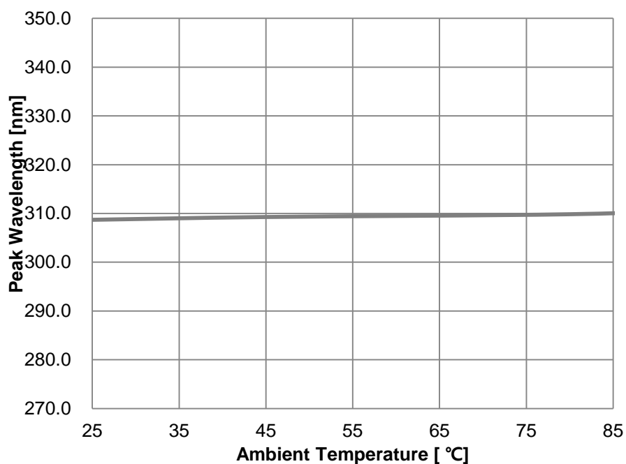
Fig 6. Ambient Temperature vs. Peak Wavelength, I_F=150\text{mA}
