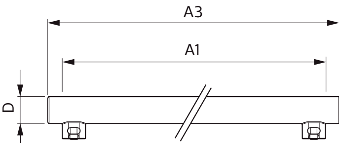
LED 220-240V 3.5-60W 375lm 2700K S14S
